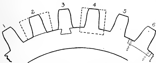
FIG. 559. METHODS OF ATTACHING SPUR GEAR TEETH.
